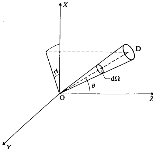
1.14 The geometry of scattering. The detector D subtends an element of solid angle d\Omega at the scattering centre O . The polar coordinates of OD are (\theta, \phi) . The incident beam is directed along the Z axis so that \theta and \phi are the scattering angles.
